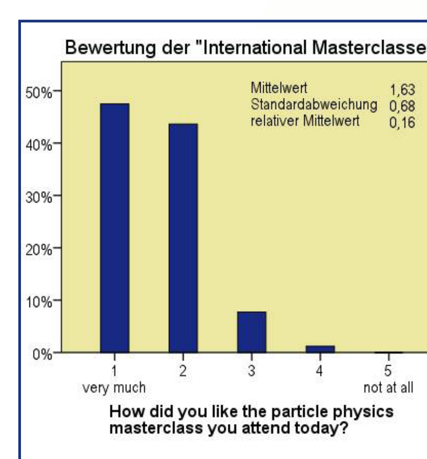
Diagramm 2 - Evaluation der International Masterclasses „Hands on Particle Physics“ (2005)
