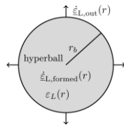
Fig. 9: A localizable and stationary portion of relative additional volume \varepsilon_L in its own system.
