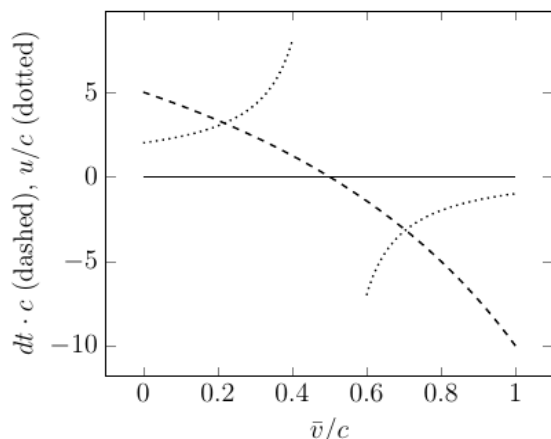
Fig. 2: Required time dt \cdot c (dashed) and velocity \frac{u}{c} (dotted) as a function of the velocity \bar{v}/c in the example proposed by Einstein (1907, p. 381). Hereby, for instance, w = 2c and dL = 10 m have been chosen. At \bar{v}/c = \frac{1}{2} , the velocity \frac{u}{c} diverges, and the time dt becomes zero. At \bar{v}/c > \frac{1}{2} , the velocity \frac{u}{c} as well as the time dt become negative: We interpret that case as follows: The object moves to the left and might have been at the point B in the past, accordingly, dt < 0 .
