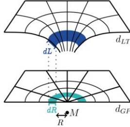
Fig. 2: In the vicinity of M or M_{eff} , the radial increment dL of d_{LT} is increased with respect to the original increment dR that would occur in the limit M to zero.
