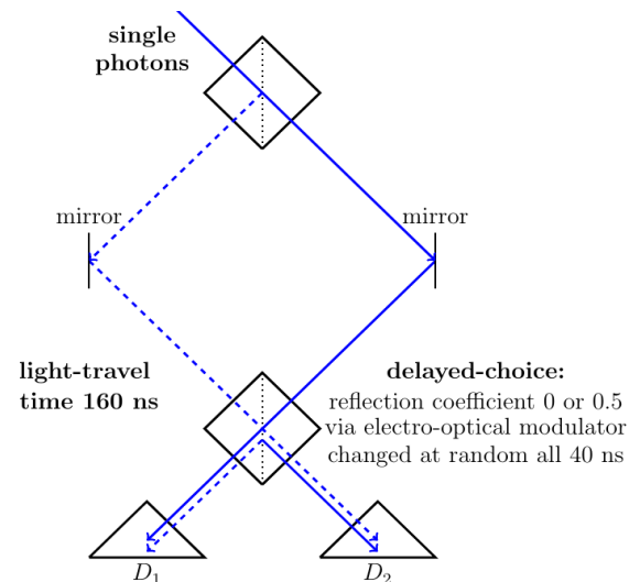
Fig. 4: Mach-Zehnder Interferometer: The second beam splitter is switched at random from reflectivity 0 to 0.5 and vice versa.
