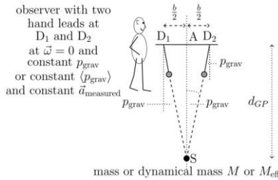
Fig. 6: Measurement of gravitational parallax distance d_{GP} via the angle of gravitational parallax p_{grav} : D_1, D_2 and S form an isosceles triangle D_1 D_2 S . The base line D_1 D_2 has the centre A . An effective mass M_{eff} is measured at constant measured acceleration \vec{a}_{measured} .
